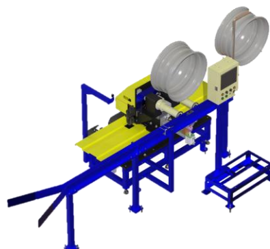
ROTARY HANGER MACHINE
