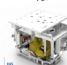
JIG LEAK TEST
